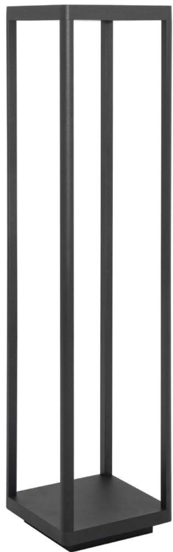
SURF - 9176102 Anthracite Die-Casting Aluminium LED 10 Watt 493Lm 3000K 200-240 Volt 50Hz Beam Angle 108° IP65 L: 18 W: 18 H: 80 cm LED IP65 WARM WHITE
